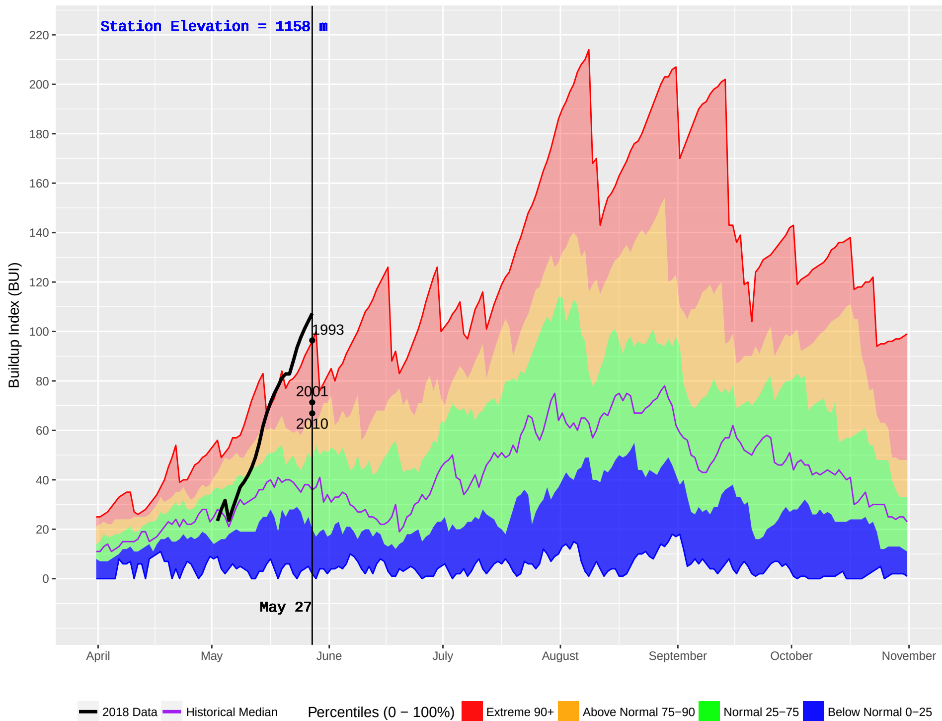
LONE BUTTE (218) : Historical (1987–2016) and Current (2018) Noon Buildup Index (BUI)
