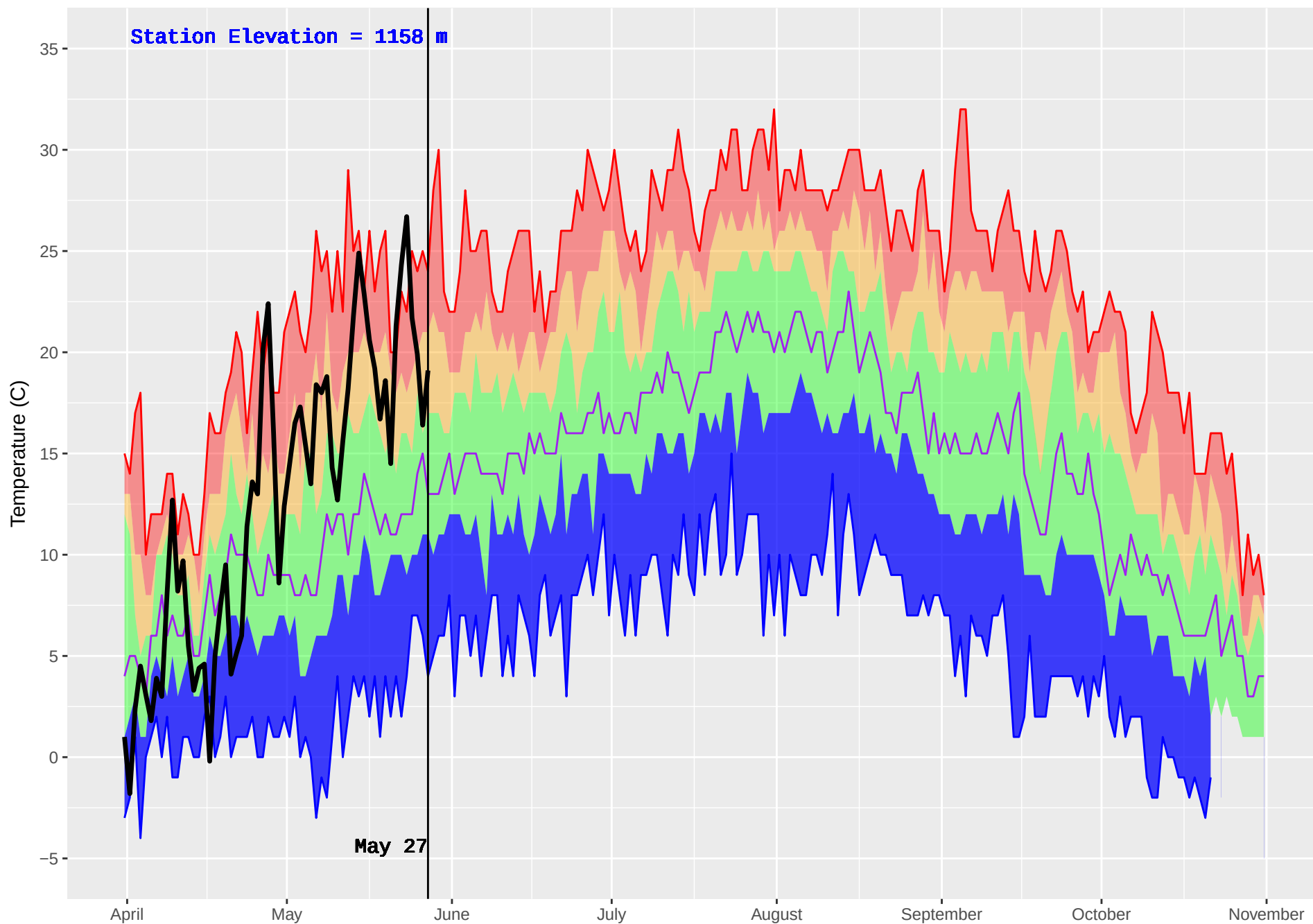
LONE BUTTE (218) : Historical (1987–2016) and Current (2018) Noon Temperature
