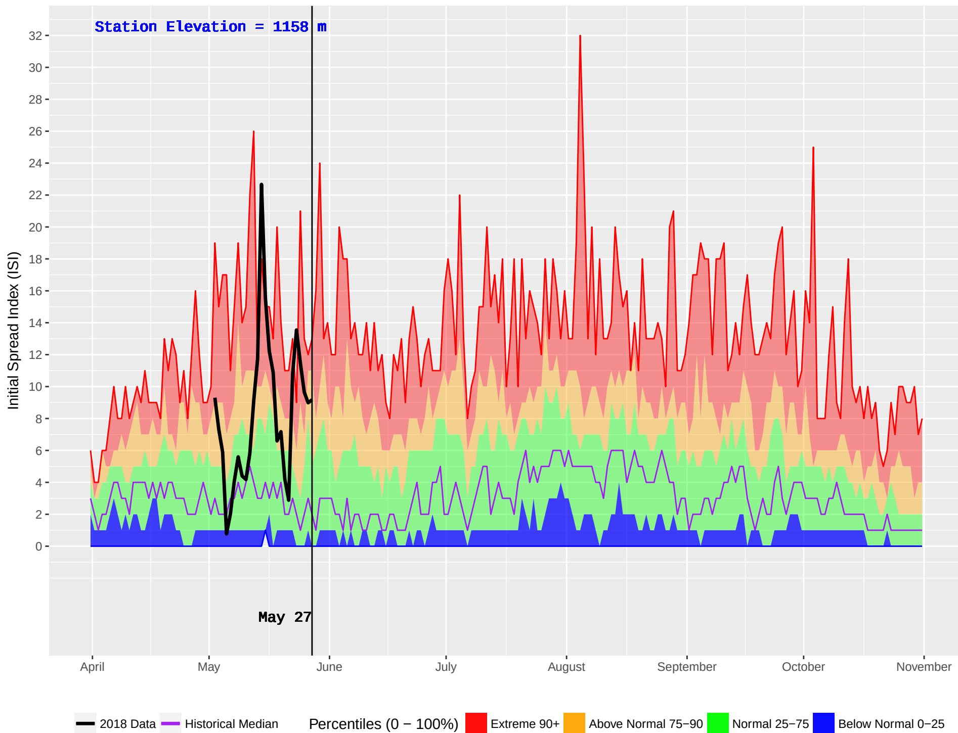
LONE BUTTE (218) : Historical (1987–2016) and Current (2018) Noon Initial Spread Index (ISI)
