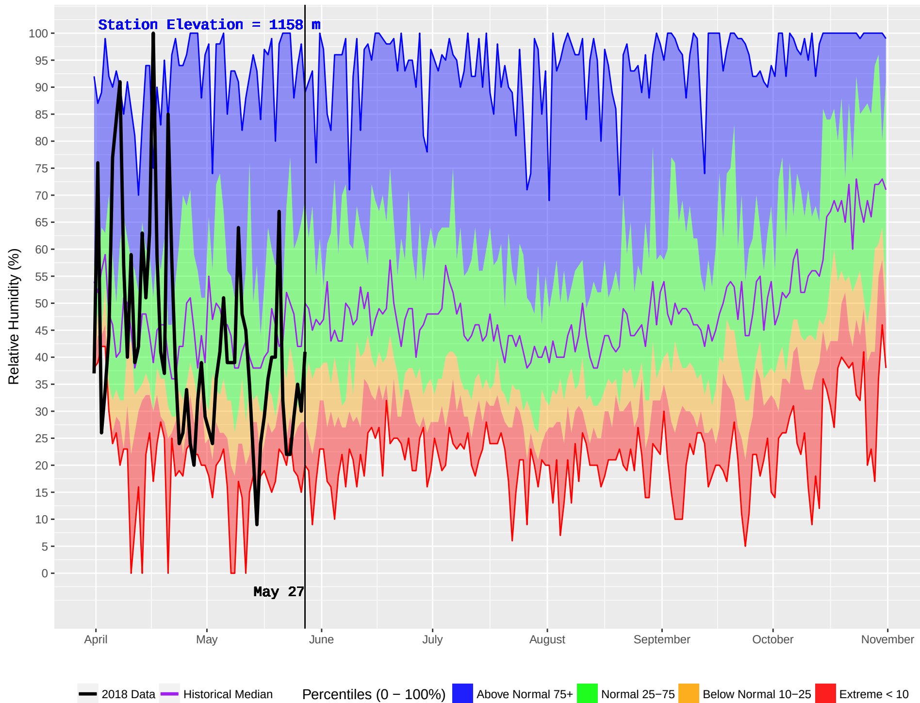
LONE BUTTE (218) : Historical (1987–2016) and Current (2018) Noon Relative Humidity
