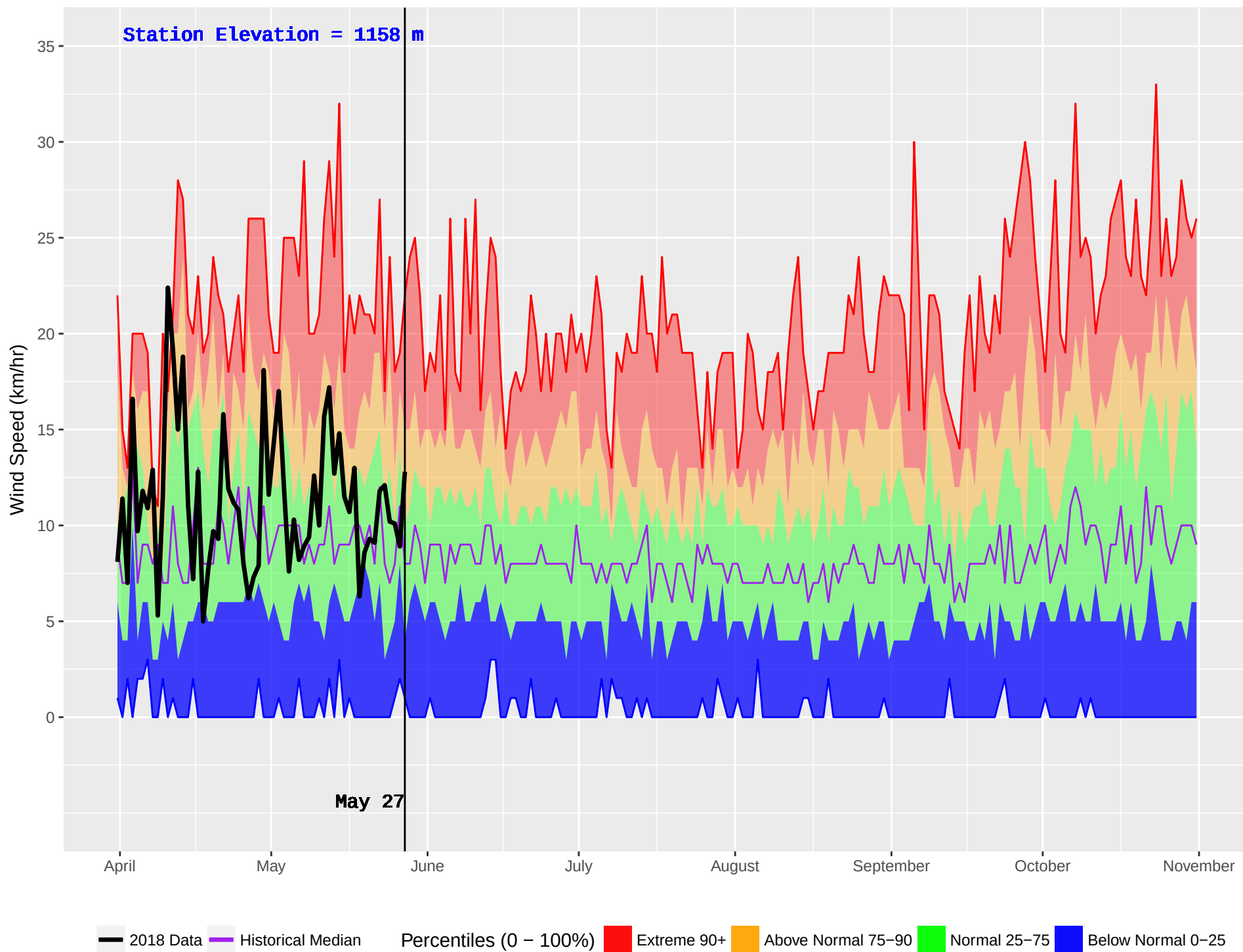
LONE BUTTE (218) : Historical (1987–2016) and Current (2018) Noon Wind Speed
